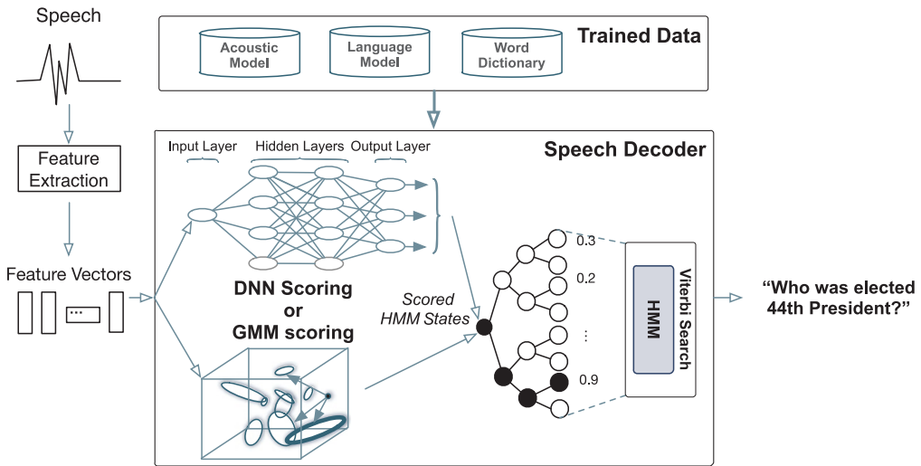
Fig. 4. ASR pipeline.
